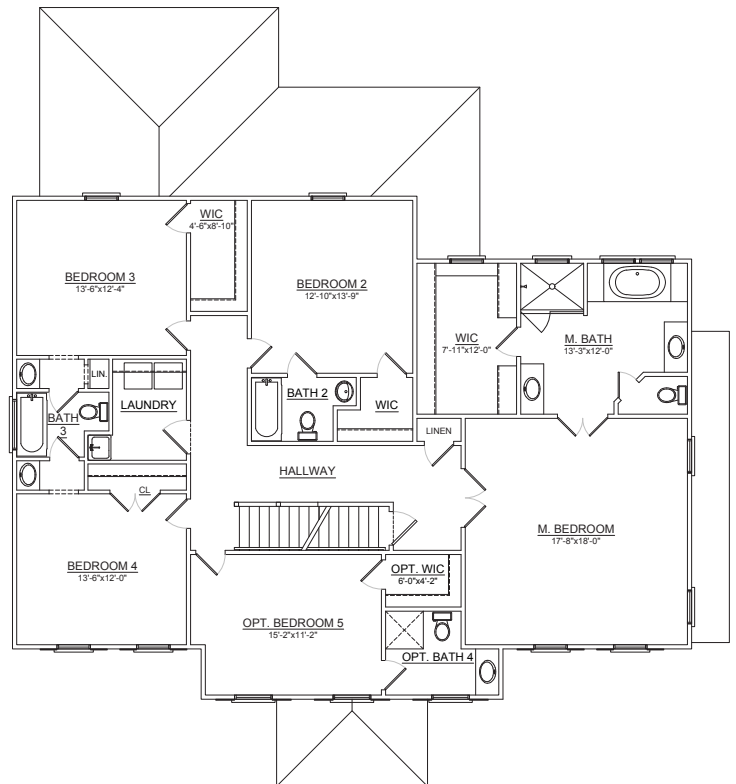
Second Floor (STANDARD)
